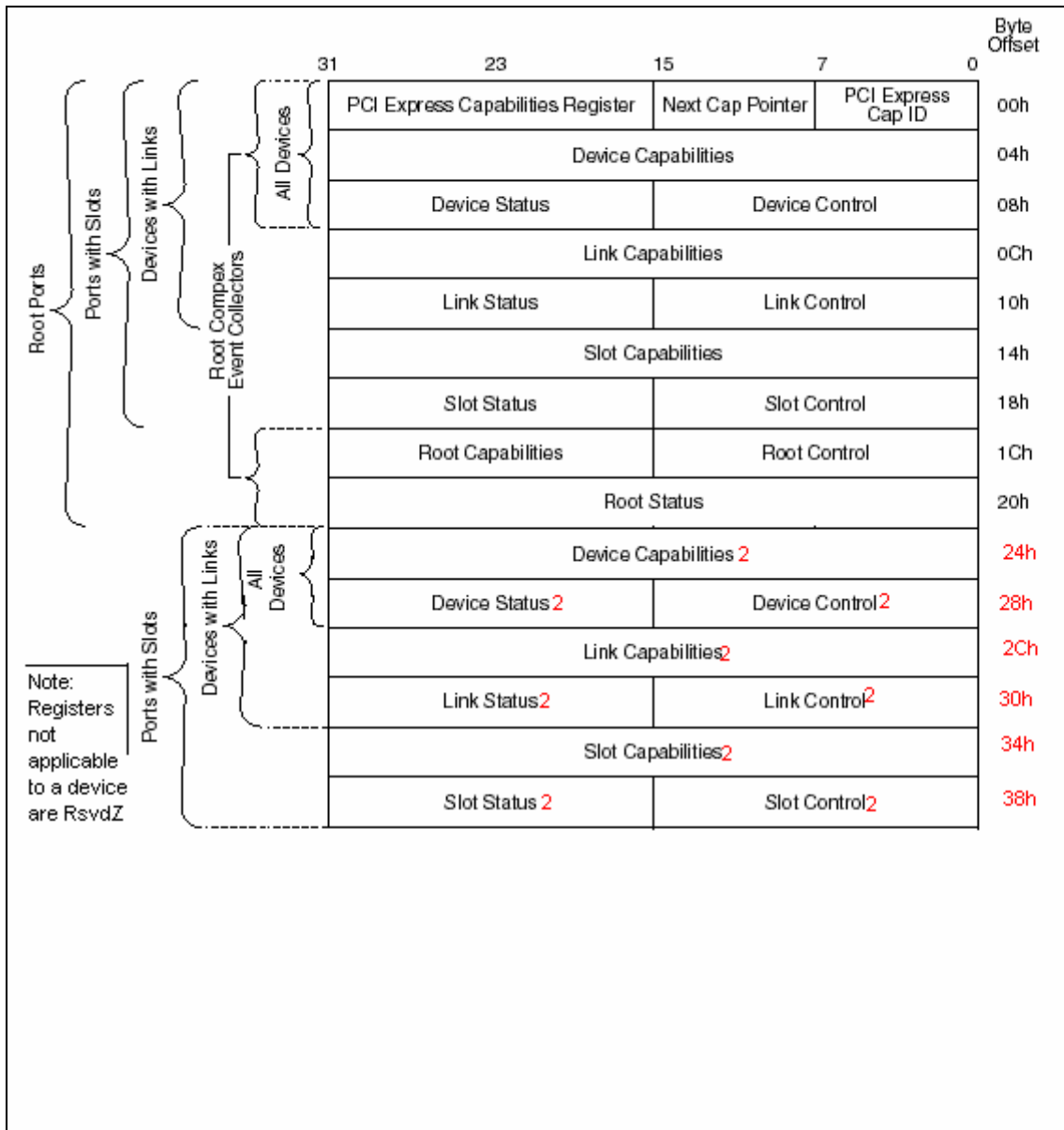
Figure 7-9: PCI Express Capability Structure
