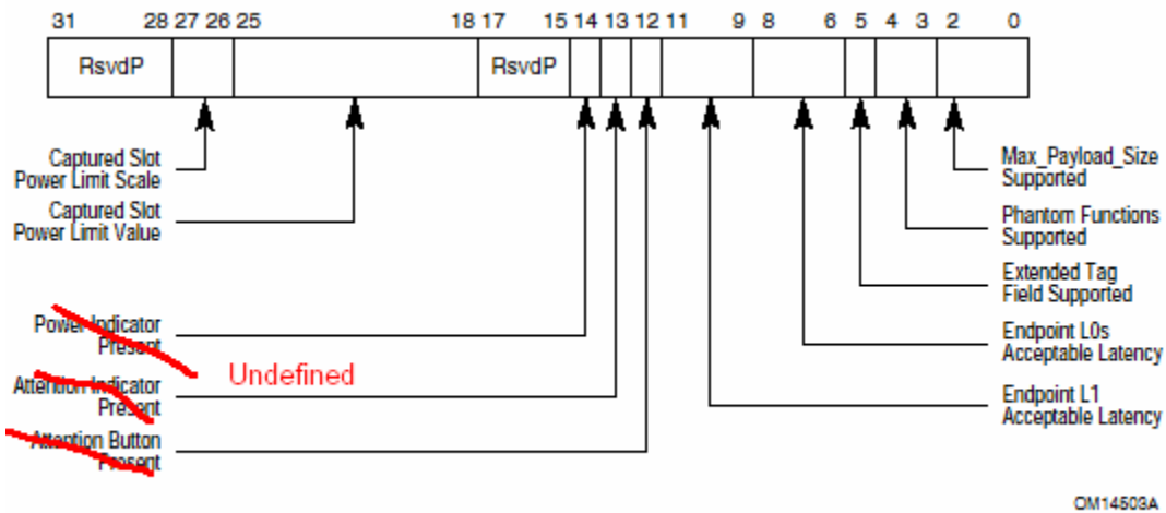
Figure 7-13: Device Capabilities Register
