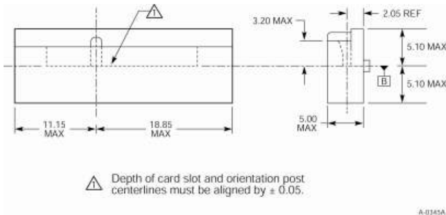
Figure 2-12: PCI Express Full-Mini and Half-Mini Card System Connector
