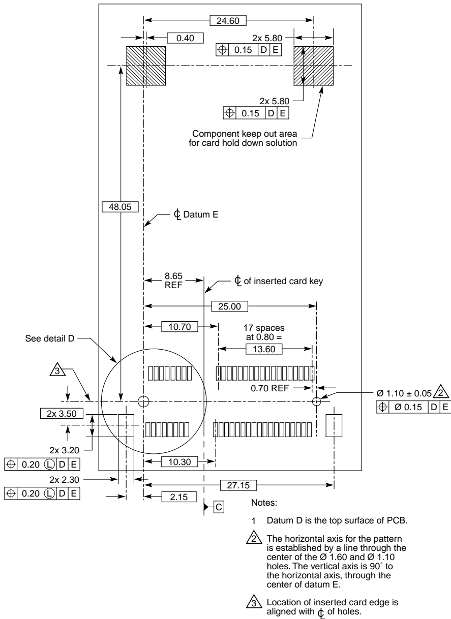
Figure 2-15: Recommended System Board Layout for Full-Mini-Only Socket
