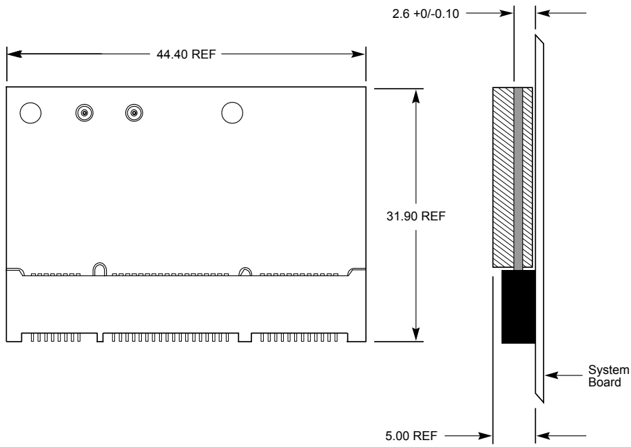
Figure 2-3: Display-Mini Card Form Factor (Wireless Example Application Shown)
