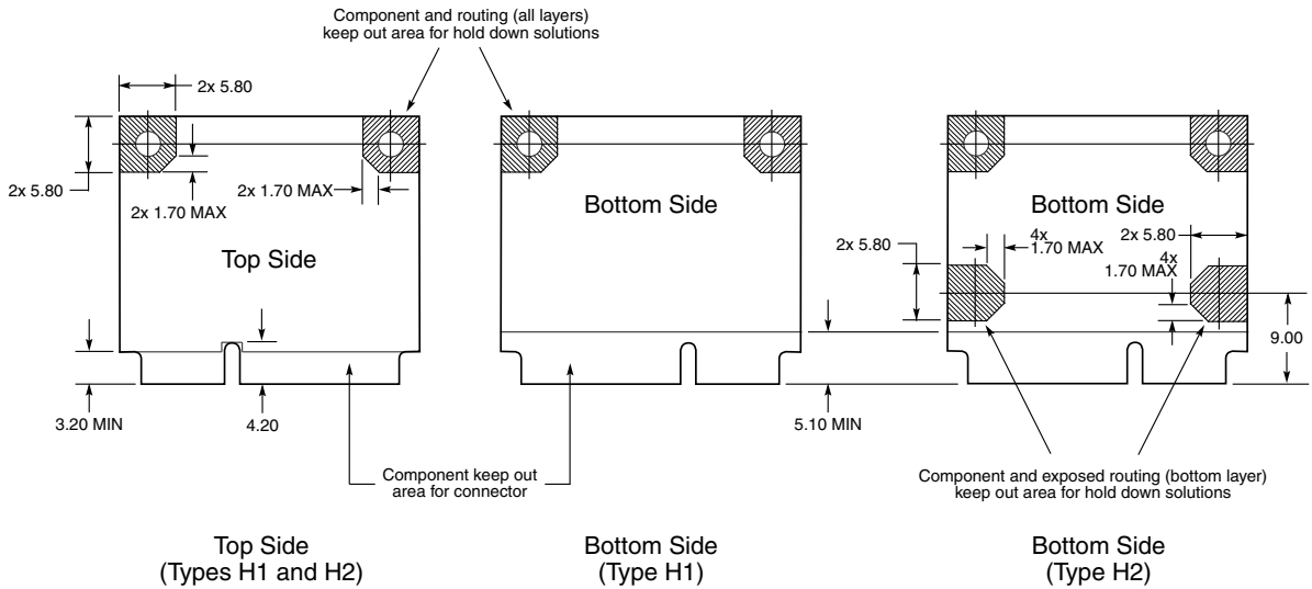
Figure 2-10: Card Component Keep Out Areas for Half-Mini Cards
