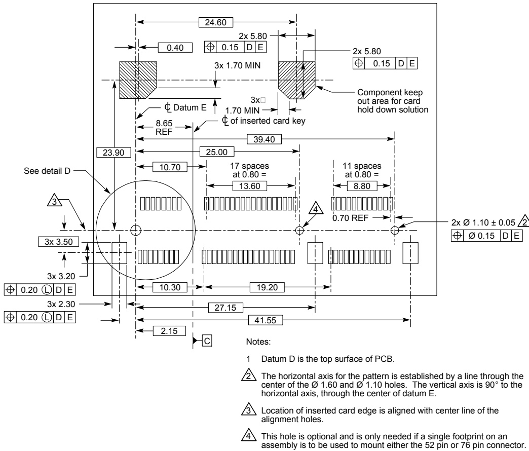
Figure 2-20: Recommended System Board Layout for Dual-Use Display/Half-Mini Card Socket
