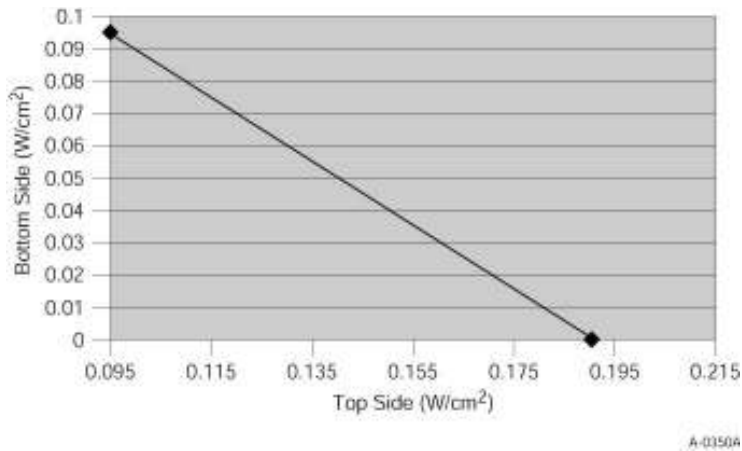
Figure 2-24: Power Density Uniform Loading at 80 Percent Coverage
