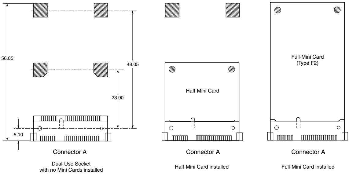
Figure 2-18: Dual-Use Full/Half-Mini Card Socket
