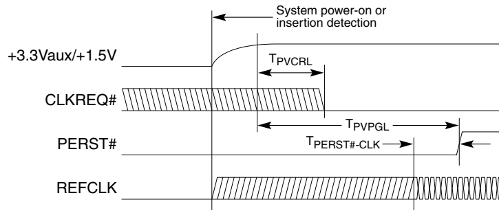
Figure 3-1: Power-Up CLKREQ# Timing
