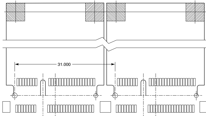
Figure 2-23: Recommended System Board Layout ( Full and Half-Mini Card Side-by-Side Spacing)
