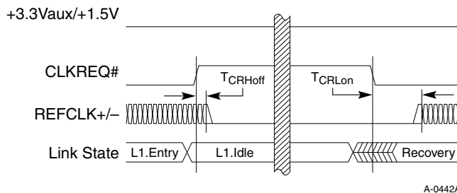
Figure 3-2: CLKREQ# Clock Control Timings
