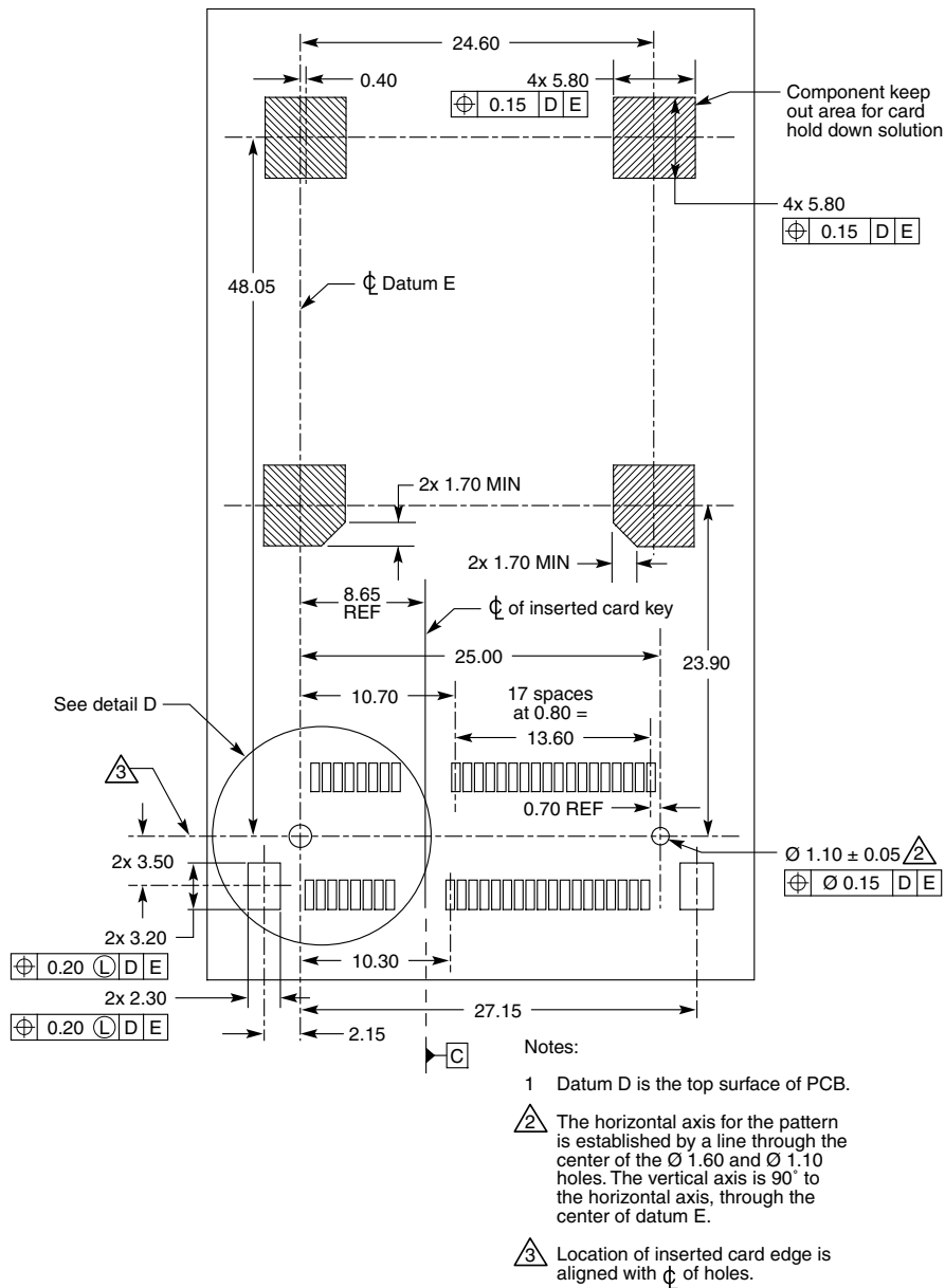
Figure 2-19: Recommended System Board Layout for Dual-Use Full/Mini Card Socket
