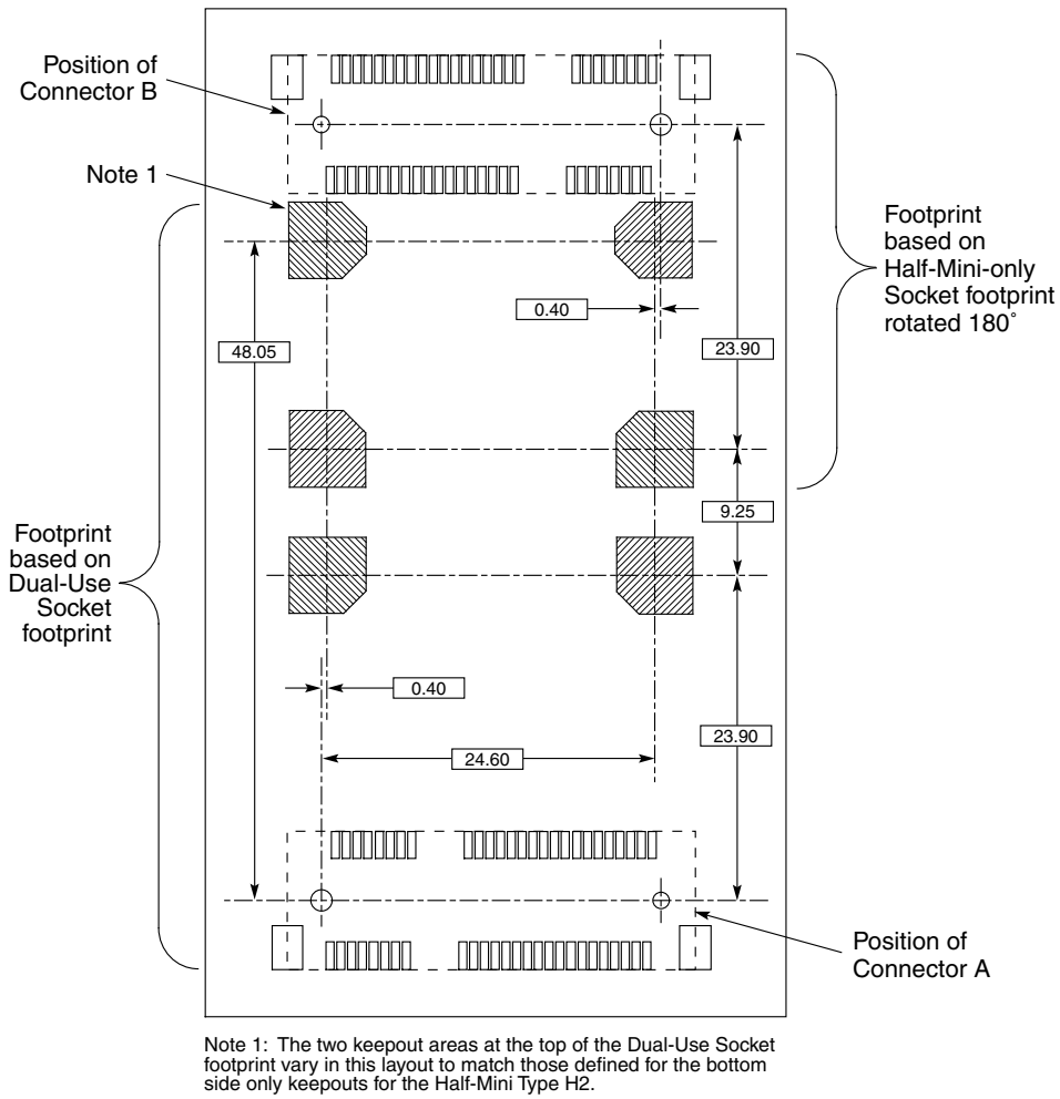
Figure 2-22: Recommended System Board Layout for Dual Head-to-Head Sockets
