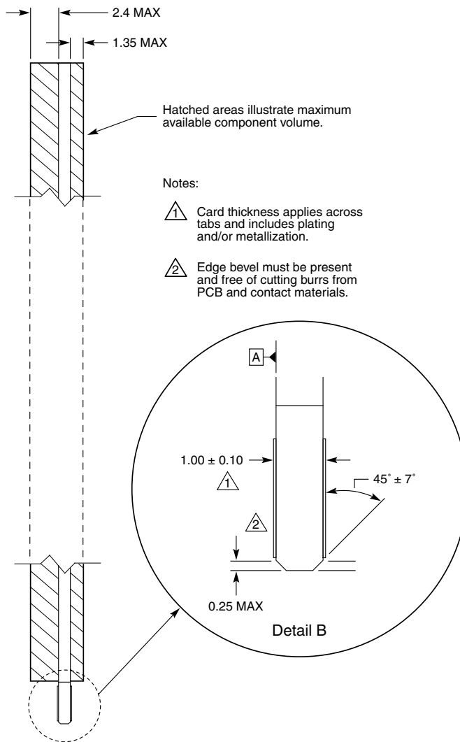
Figure 2-8: Card Edge
