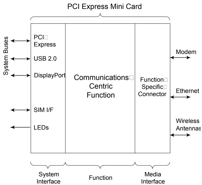
Figure 1-2: Logical Representation of the PCI Express Mini Card Specification
