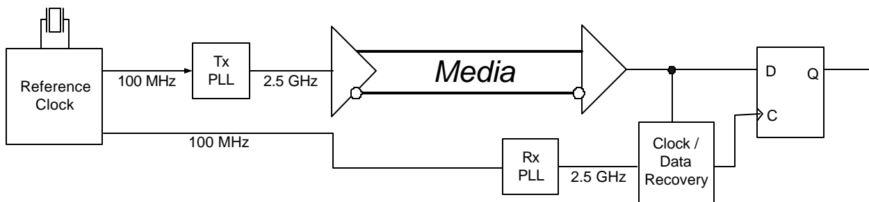
Figure 2: Physical Link Jitter Architecture
